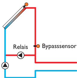
Variante Pumpe:
